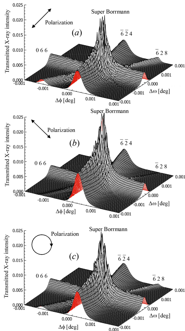
図 L.10 Transmittance of X-rays around the condition that \bar{6} \bar{2} 4 , \bar{6} \bar{2} 8 and 0 \bar{6} 6 Laue reflected X-rays are simultaneously strong. \Delta\omega and \Delta\phi are angular deviation around [\bar{2} \bar{1} 1] and [0 \bar{1} 1] axes from the exact four-beam condition.
