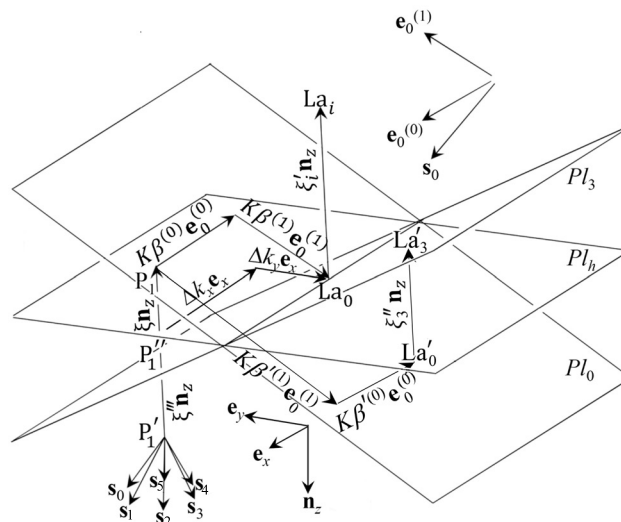
図 L.1 Geometry around the Laue point La_0 . Pl_0 and Pl_3 are planes whose distance from H_0 and H_3 is K . Pl_h is a plane normal to \mathbf{n}_z (downward surface normal). The Laue point La_0 and point P'_1 exist on Pl_h . Pl_i ( i \neq \{0, 3\} ) were not drawn for simplicity. La_i and La'_i are points whose distance from H_i ( i \in \{0, 1, \dots, n-1\} ) is K . P'_1 is the initial point of wavevector of the Bloch wave. P'_{1,k} that appears in equation (L.51) is the k th numbered P'_1 i.e., the initial point of wavevector of the k th numbered Bloch wave where k \in \{1, 2, 3, \dots, 2n\} .
